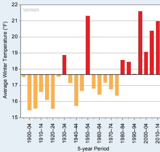
Figure 2: The observed (a) number of hot days (annual number of days with maximum temperature above 90°F), (b) number of very cold nights (annual number of days with minimum temperature below 0°F), (c) annual winter and summer temperatures, and (d) number of extreme precipitation events (annual number of events with greater than 2 inches), averaged over 5-year periods. The values in figures 2a, 2b, and 2d are averages from long-term reporting stations (seven for temperature and fifteen for precipitation). The values in figures 2c are from NCEI’s version 2 climate division dataset. The dark horizontal lines represent the long-term averages. Values for the contiguous United States (bottom panel) are also shown, where appropriate, to provide a longer and larger context. Long-term stations back to 1900 were not available for Vermont. Over the past two decades (1995–2014), Vermont has experienced the highest winter and summer temperatures and the greatest number of extreme precipitation events observed in the historical record. There is no trend in the number of hot days while the number of very cold nights has been below average over the last 10 years. Source: CICS-NC and NOAA NCEI.
