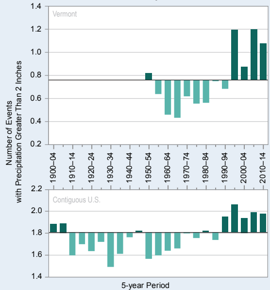
Figure 2: The observed (a) number of hot days (annual number of days with maximum temperature above 90°F), (b) number of very cold nights (annual number of days with minimum temperature below 0°F), (c) annual winter and summer temperatures, and (d) number of extreme precipitation events (annual number of events with greater than 2 inches), averaged over 5-year periods. The values in figures 2a, 2b, and 2d are averages from long-term reporting stations (seven for temperature and fifteen for precipitation). The values in figures 2c are from NCEI’s version 2 climate division dataset. The dark horizontal lines represent the long-term averages. Values for the contiguous United States (bottom panel) are also shown, where appropriate, to provide a longer and larger context. Long-term stations back to 1900 were not available for Vermont. Over the past two decades (1995–2014), Vermont has experienced the highest winter and summer temperatures and the greatest number of extreme precipitation events observed in the historical record. There is no trend in the number of hot days while the number of very cold nights has been below average over the last 10 years. Source: CICS-NC and NOAA NCEI.
