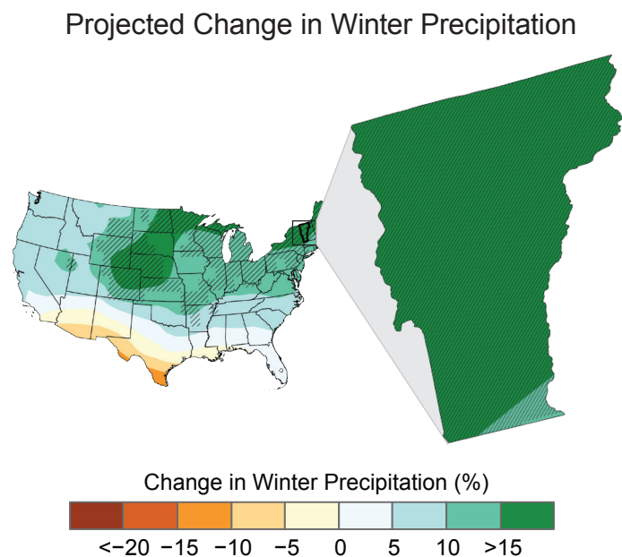
Figure 5: Projected change in winter precipitation (%) by the middle of the 21st century compared to the late 20th century under a higher emissions pathway. Hatching represents areas where the majority of climate models indicate a statistically significant change. Vermont is part of a large area of the Northeast that is expected to experience increases in winter precipitation. Source: CICS-NC and NOAA NCEI.
