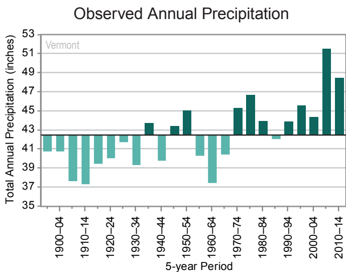
Figure 4: The observed annual precipitation for 1895–2014, averaged over 5-year periods; these values are averages from NCEI’s version 2 climate division dataset. Below average annual precipitation occurred in Vermont during the first half of the 20th century. Annual precipitation has largely remained above average since 1970. The dark horizontal line is the long-term average of 42.4 inches per year. Source: CICS-NC and NOAA NCEI.
